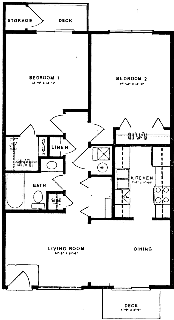
2 BEDROOMS, 1 BATH 864 sq. ft.
